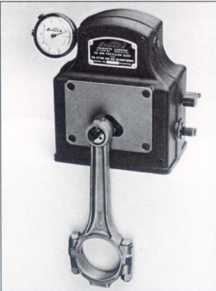
The only gage made for both clearance and press type pin fits AND THE JOURNAL END OF CON-RODS.
